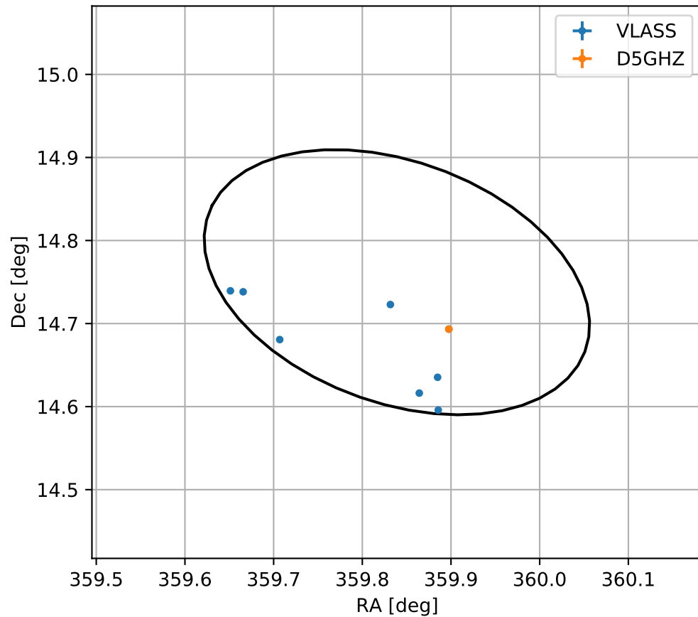
4FGL J2359.3+1444
