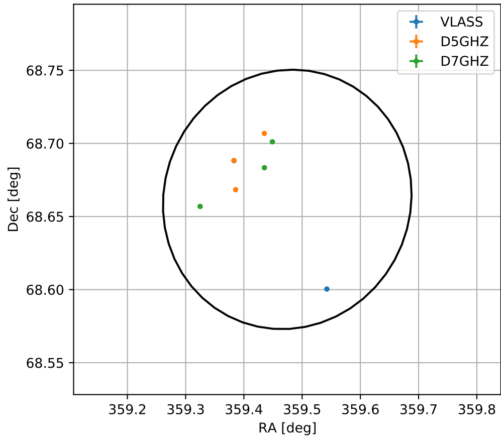
4FGL J2357.8+6839
