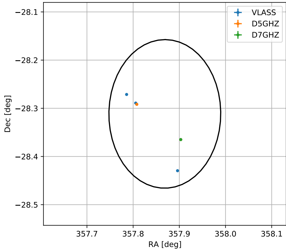
4FGL J2351.4-2818
