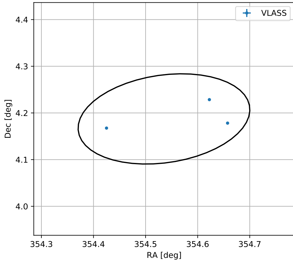
4FGL J2338.1+0411
