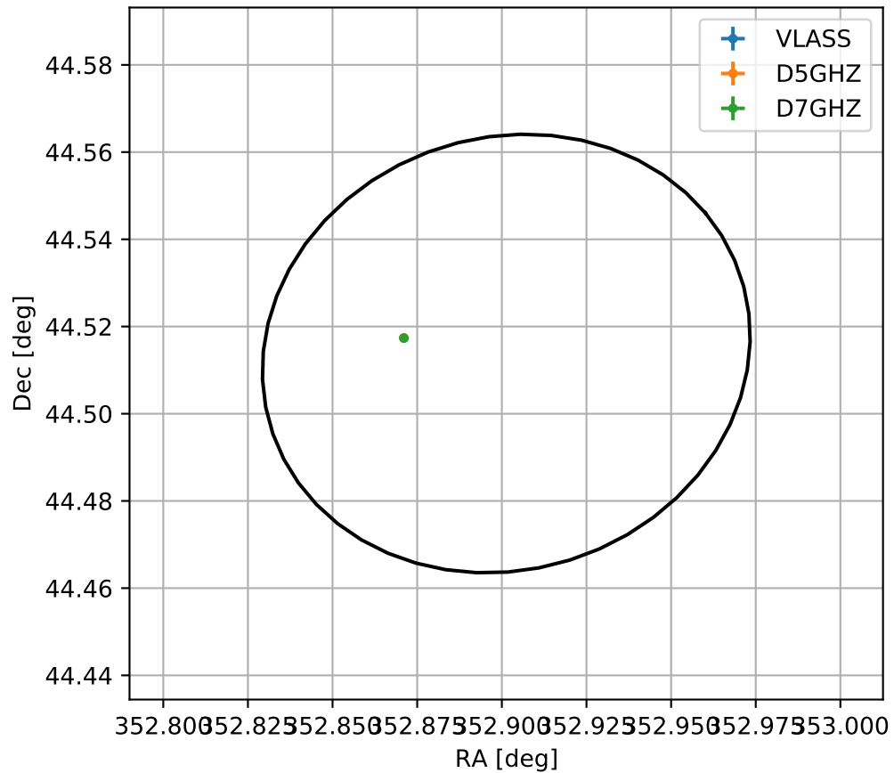
4FGL J2331.6+4430
