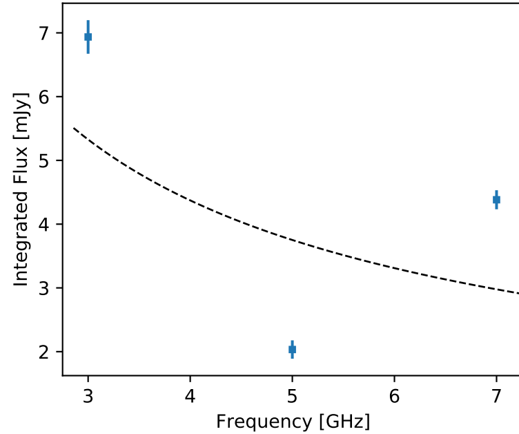
F357 J233129.05+443102.4 (unr)
