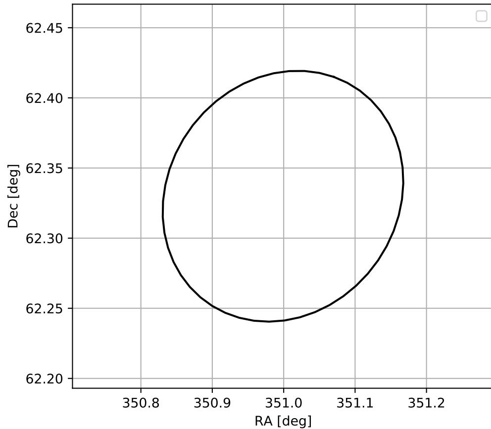
4FGL J2323.9+6219
