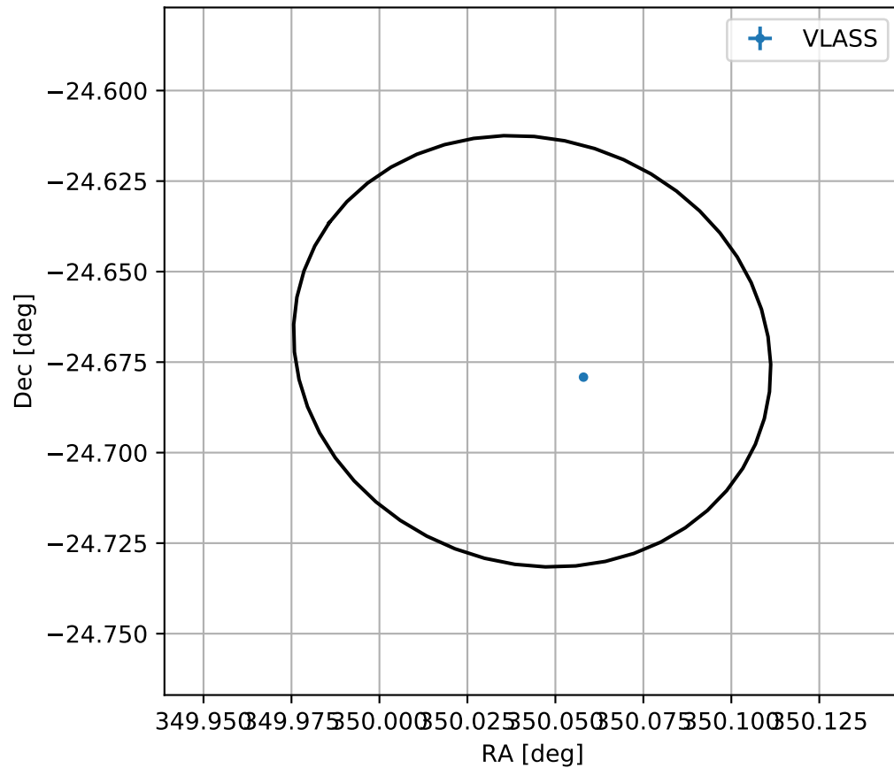
4FGL J2320.1-2440
