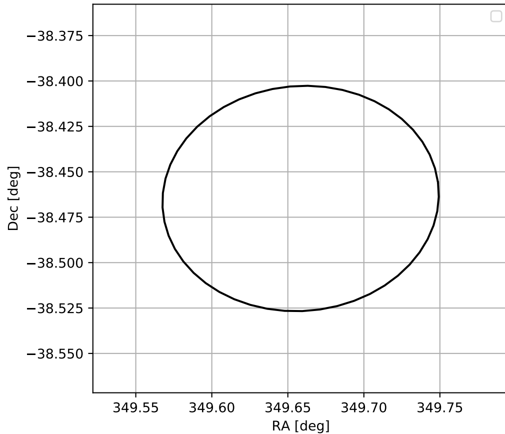
4FGL J2318.6-3827
