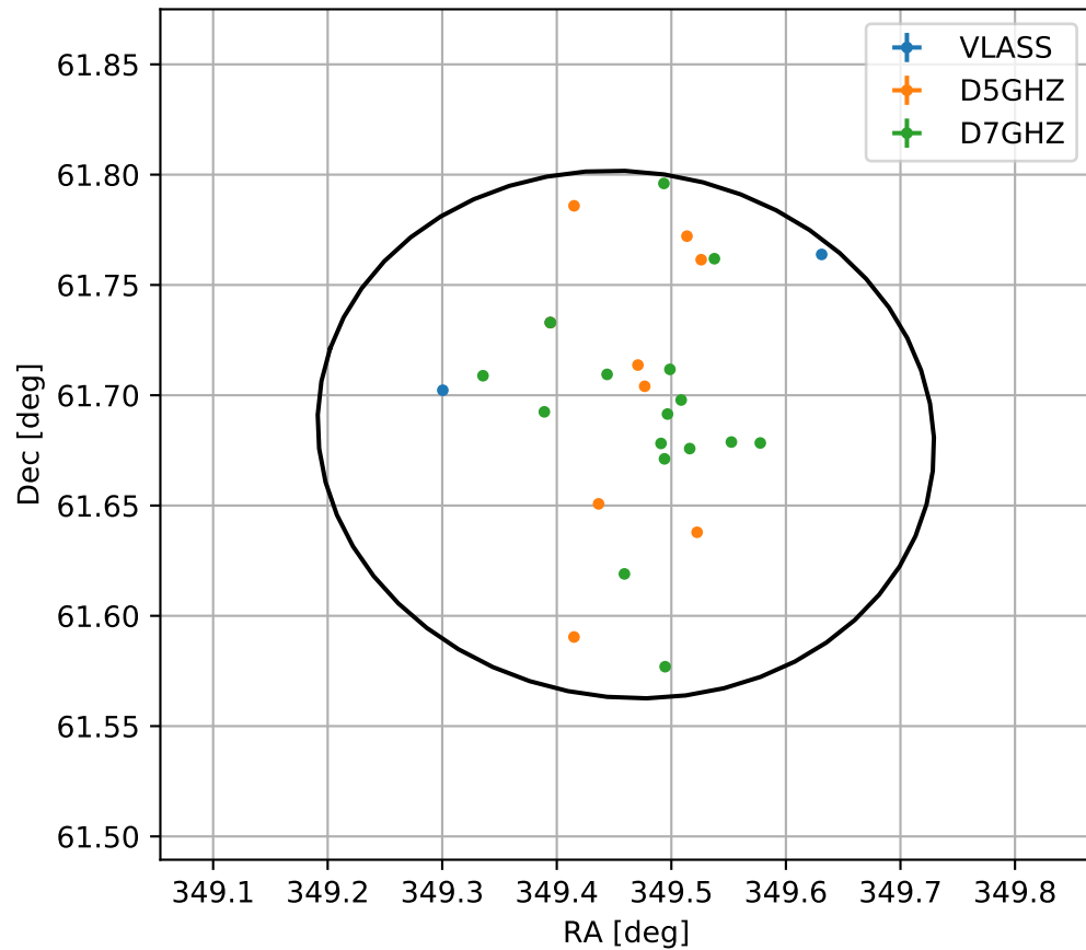
4FGL J2317.8+6140c
