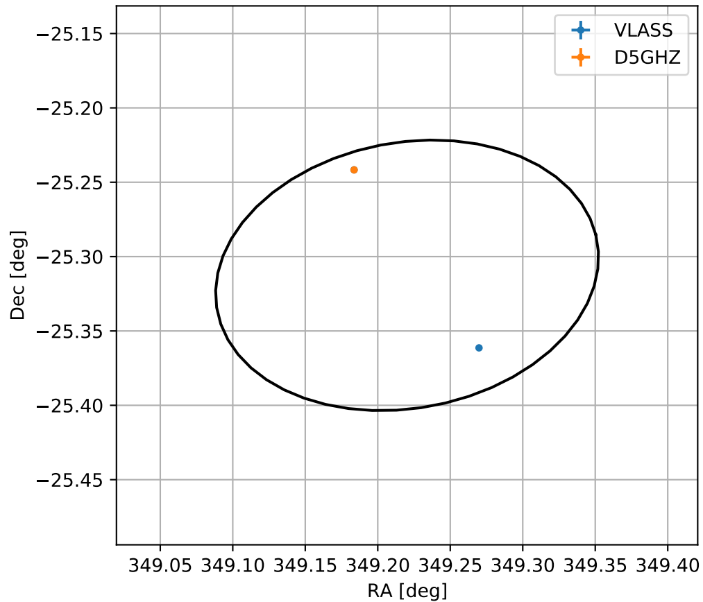
4FGL J2316.8-2518
