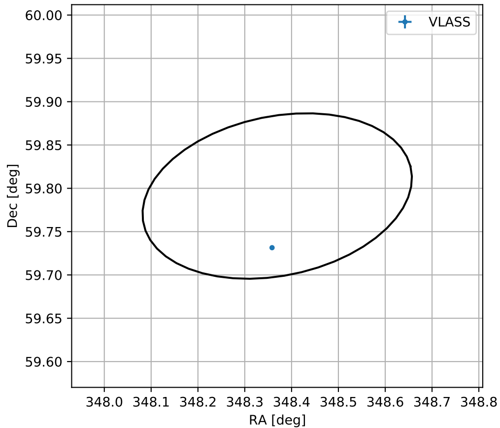
4FGL J2313.4+5947
