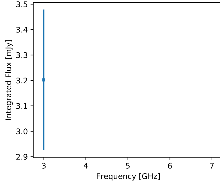
F357 J231325.99+594353.2 (unr)
