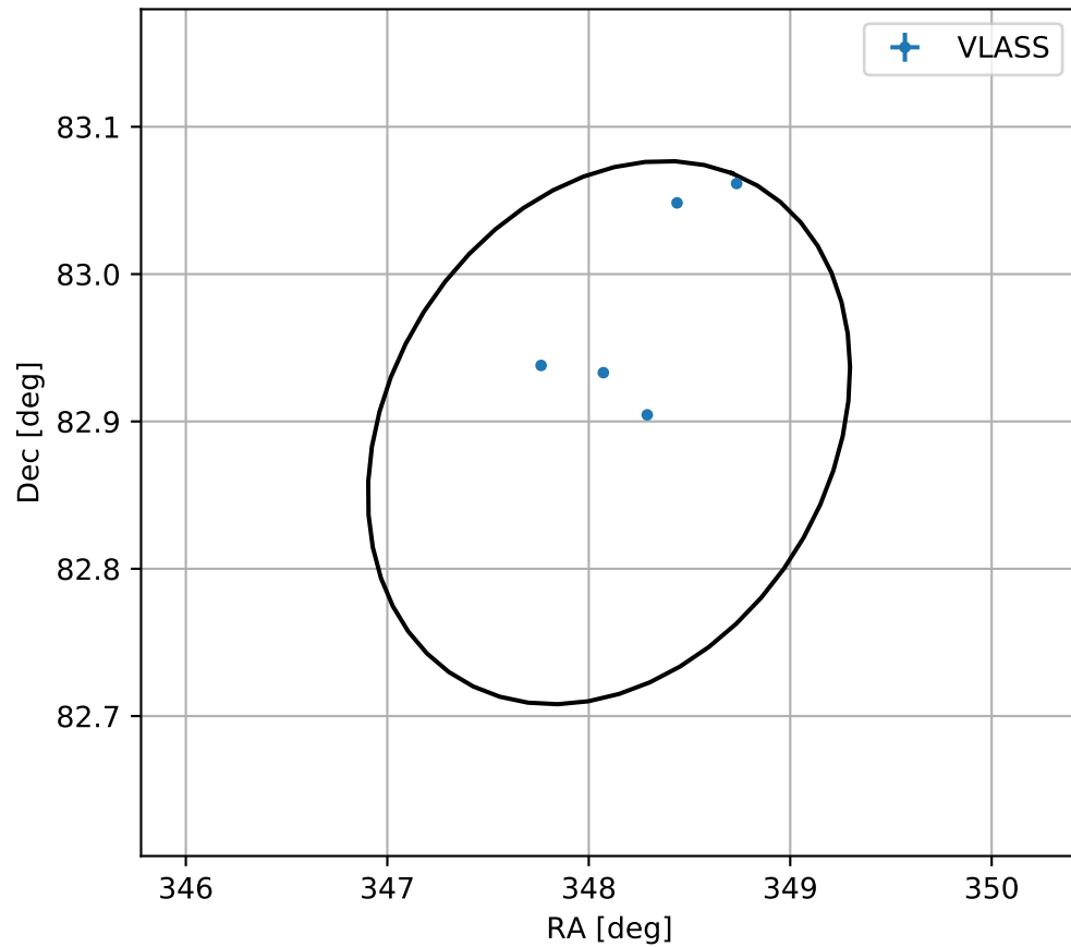
4FGL J2312.4+8253
