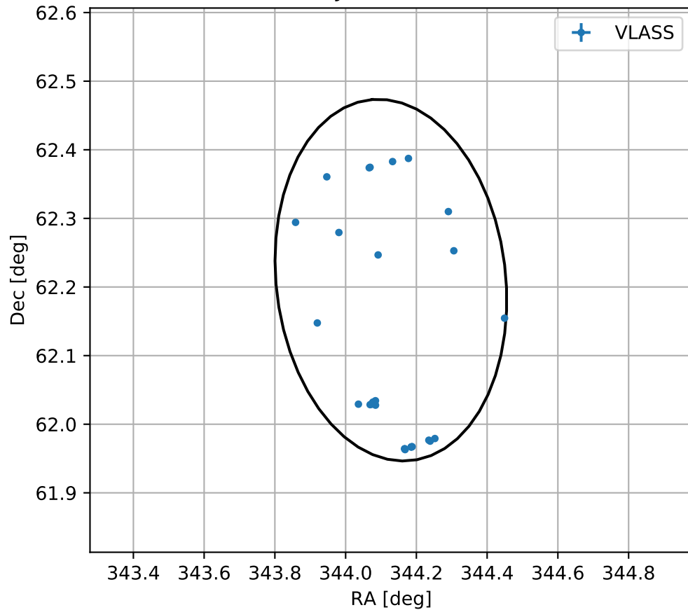
4FGL J2256.5+6212c
