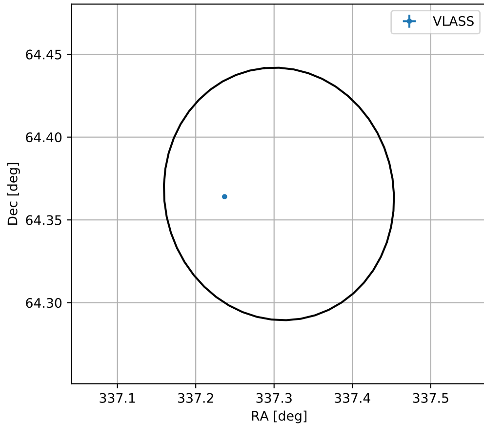
4FGL J2229.2+6421c
