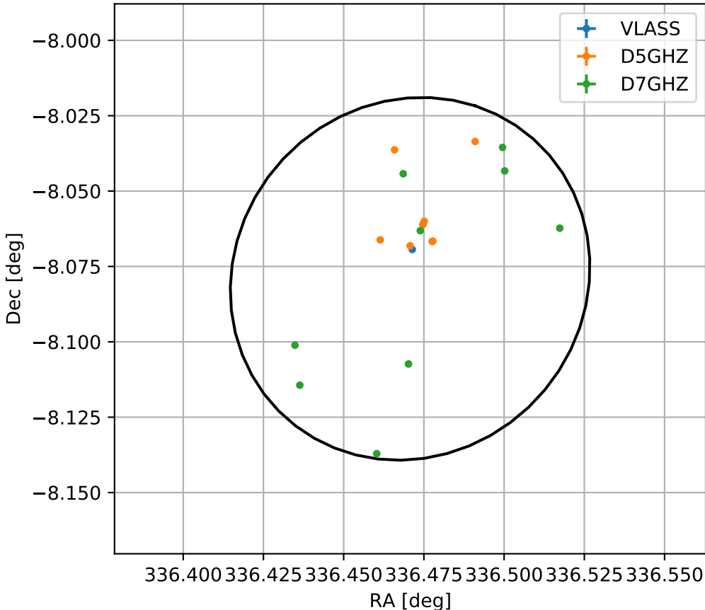
4FGL J2225.8-0804
