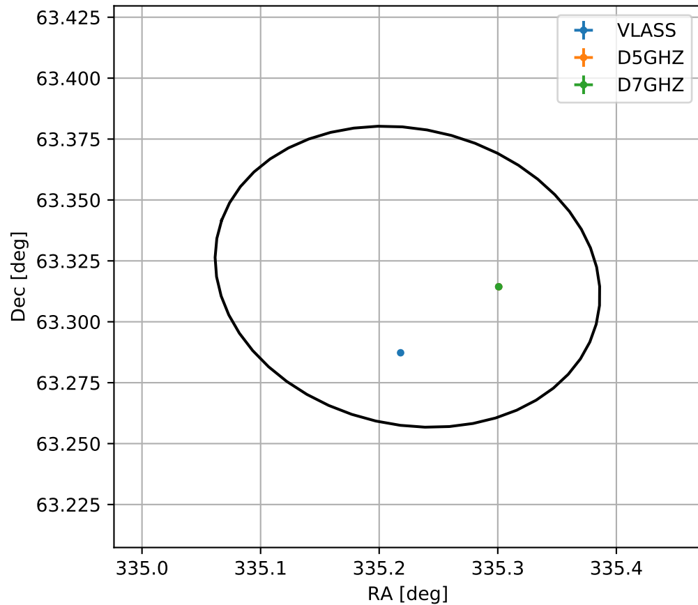
4FGL J2220.8+6319
