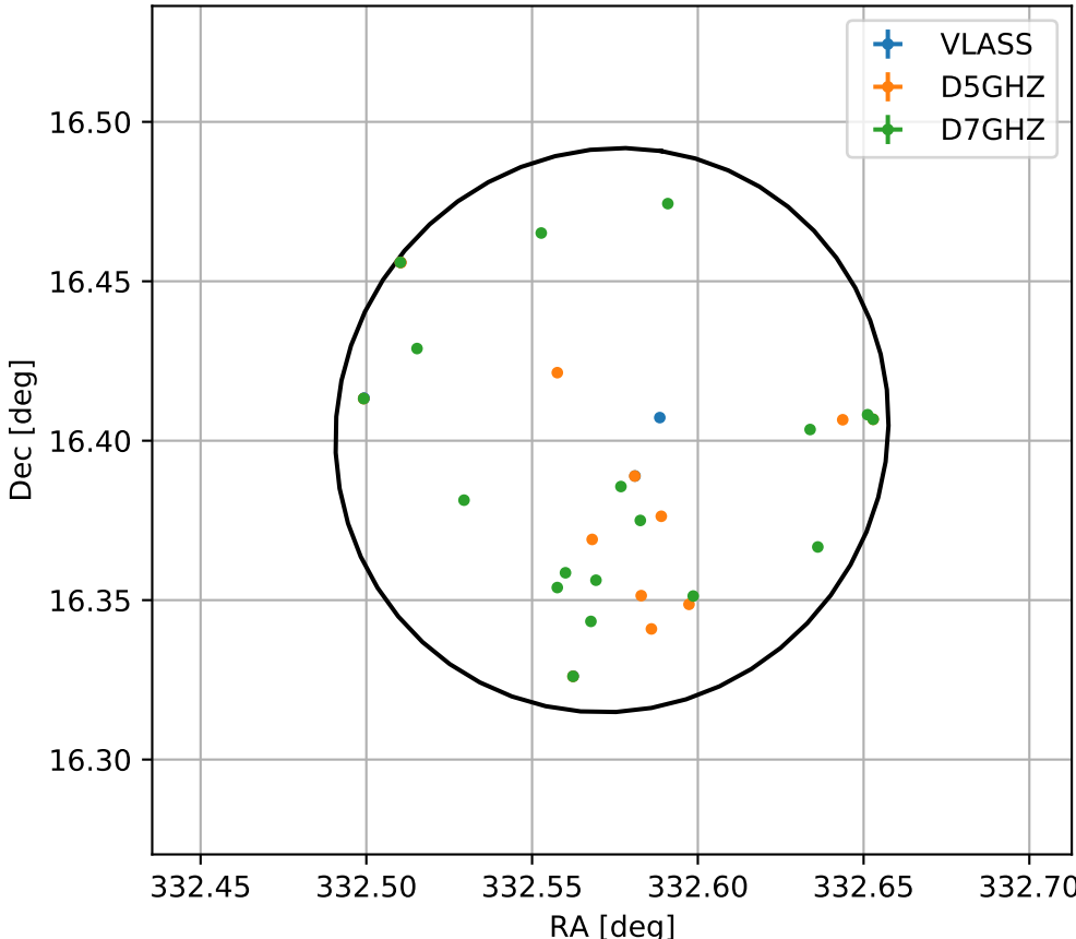
4FGL J2210.2+1624
