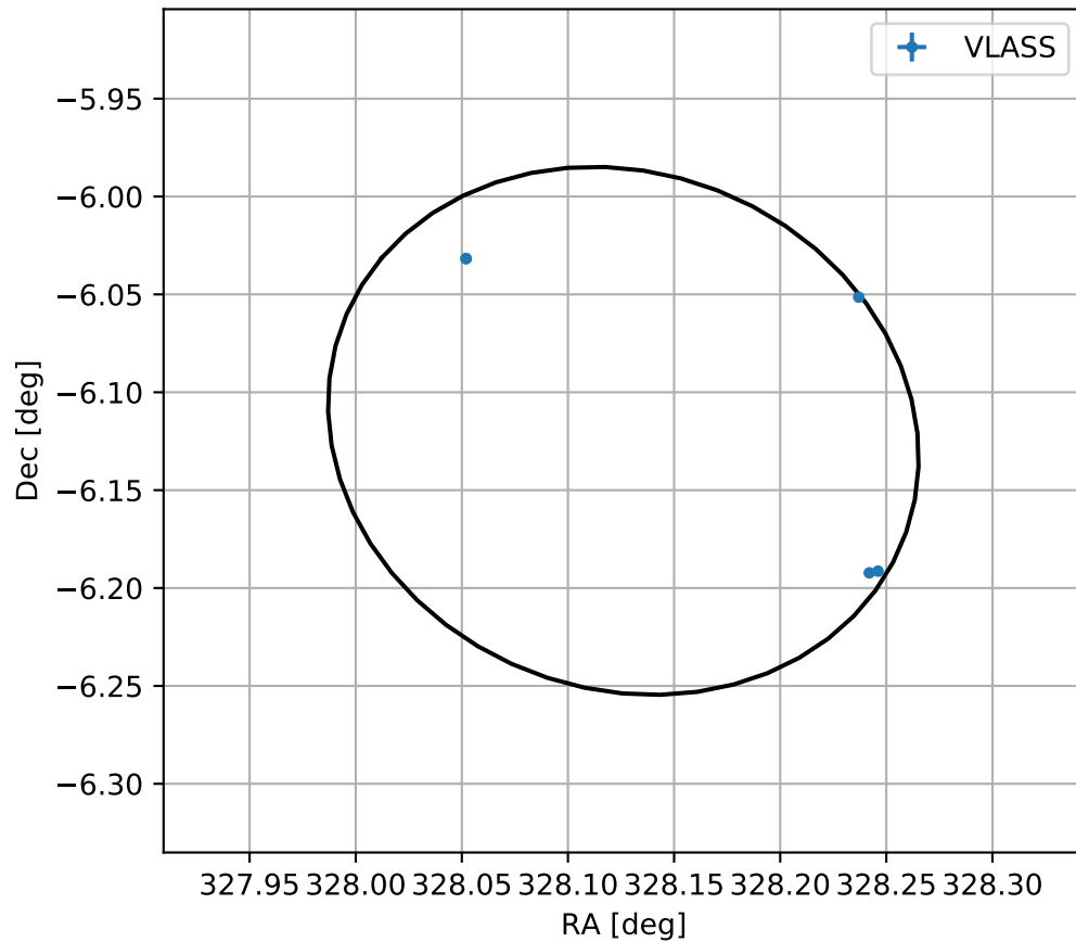
4FGL J2152.5-0607
