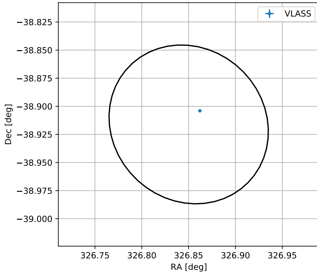
4FGL J2147.4-3854
