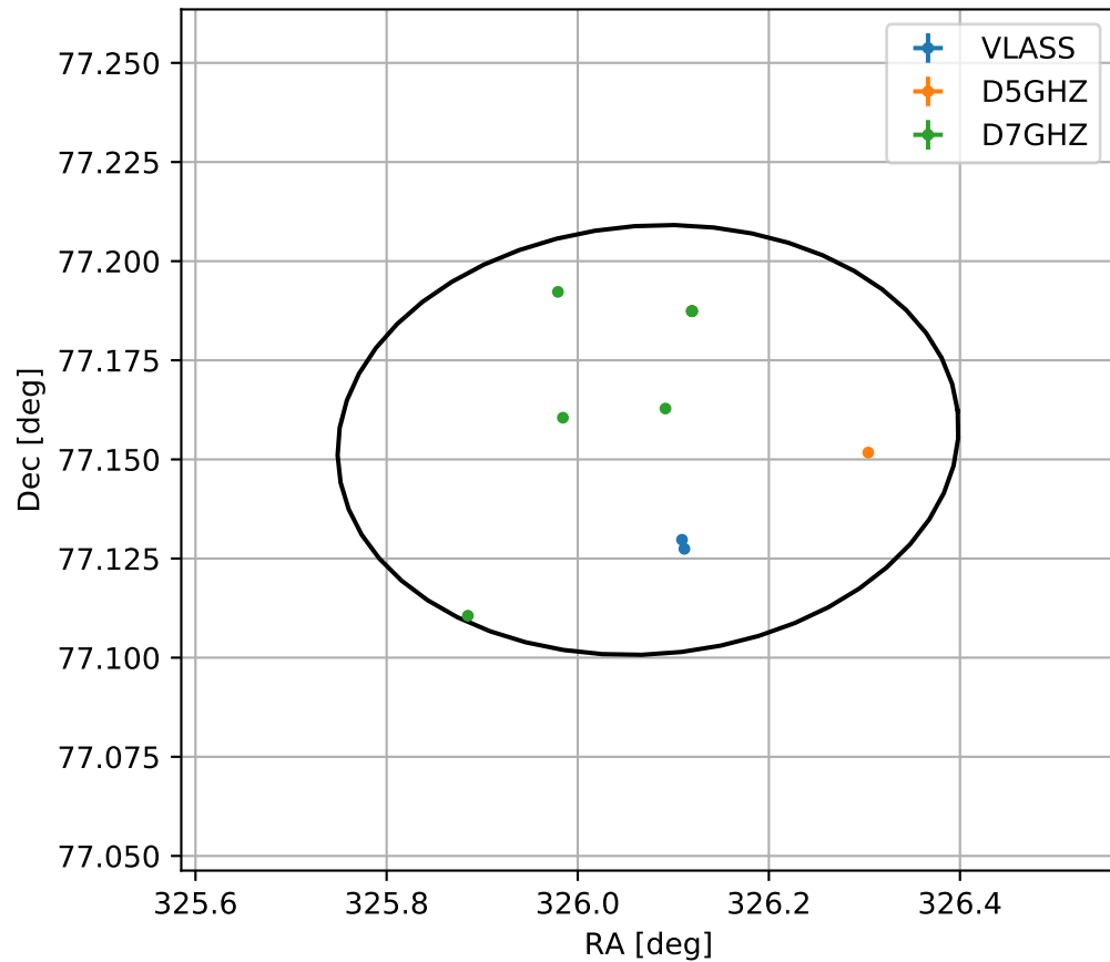
4FGL J2144.2+7709c
