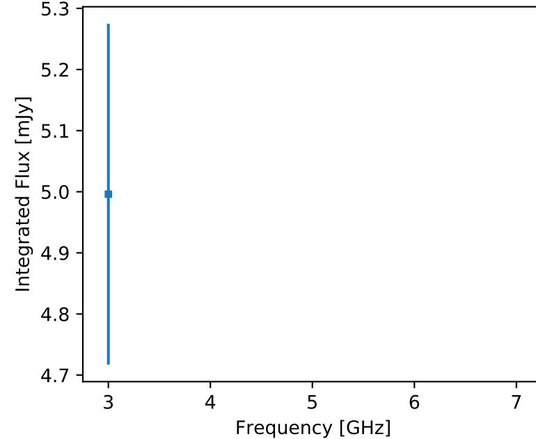
F357 J214239.80-202819.0 (unr)
