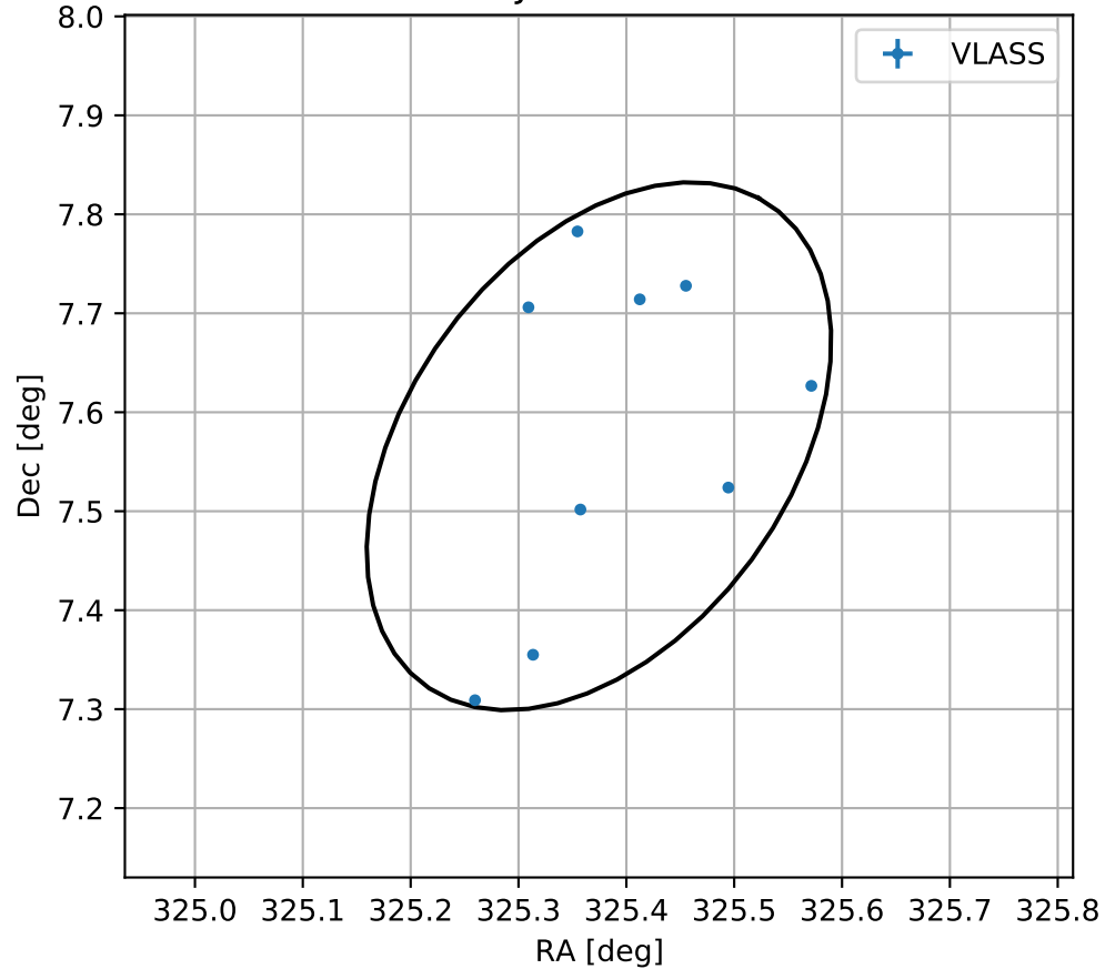
4FGL J2141.4+0733
