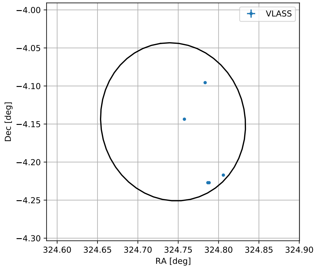
4FGL J2138.9-0408
