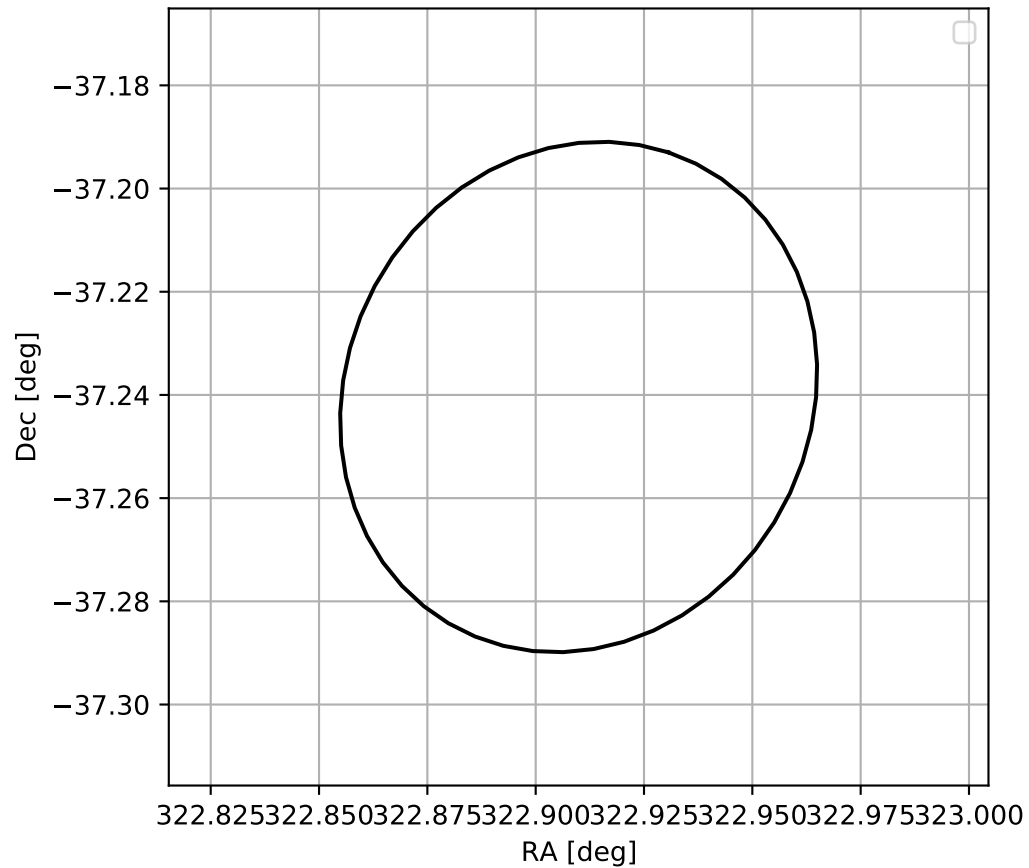
4FGL J2131.6-3714
