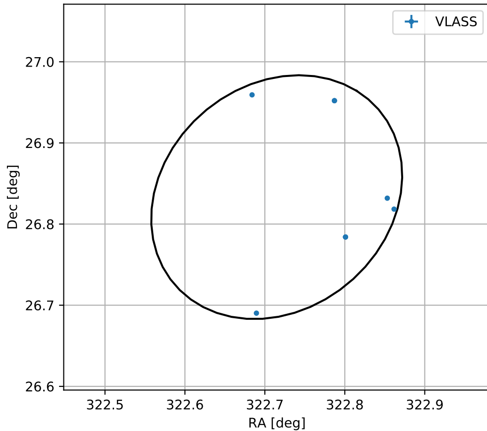
4FGL J2130.8+2649
