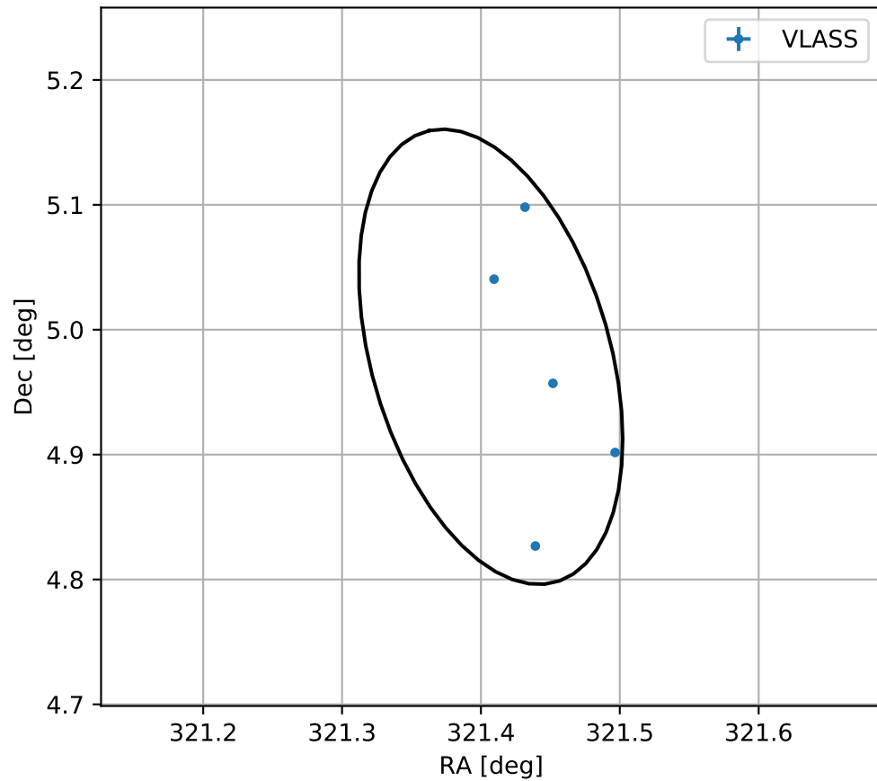
4FGL J2125.6+0458
