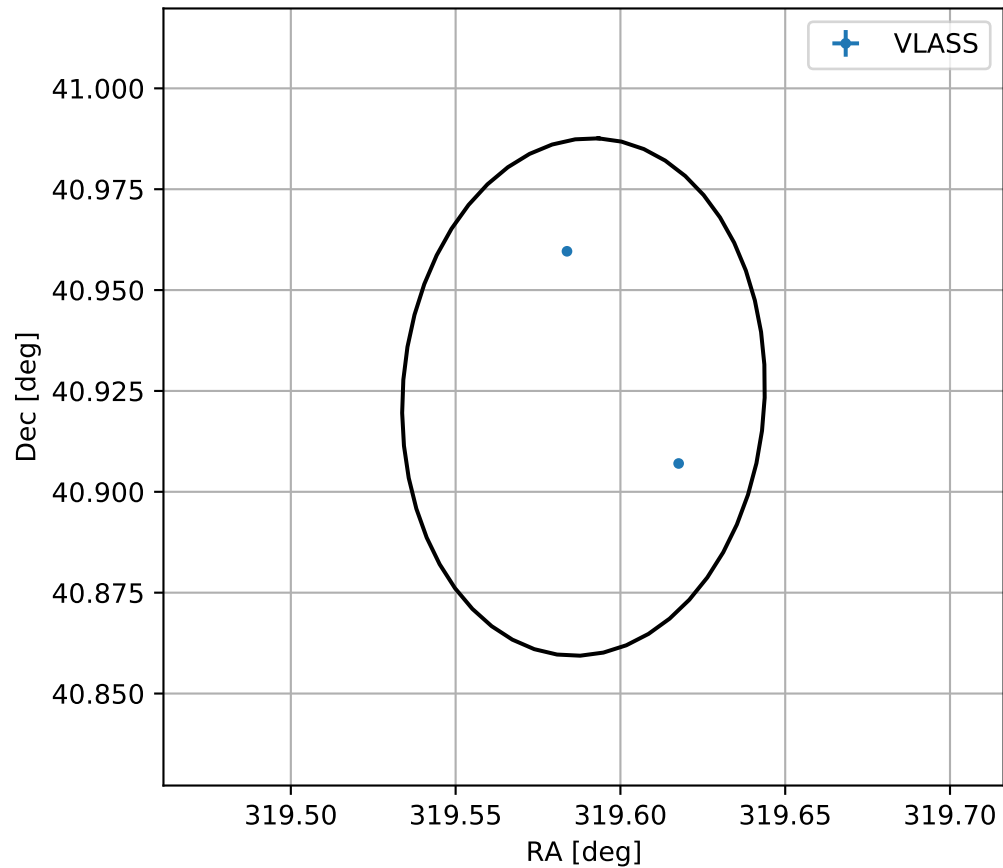
4FGL J2118.3+4055
