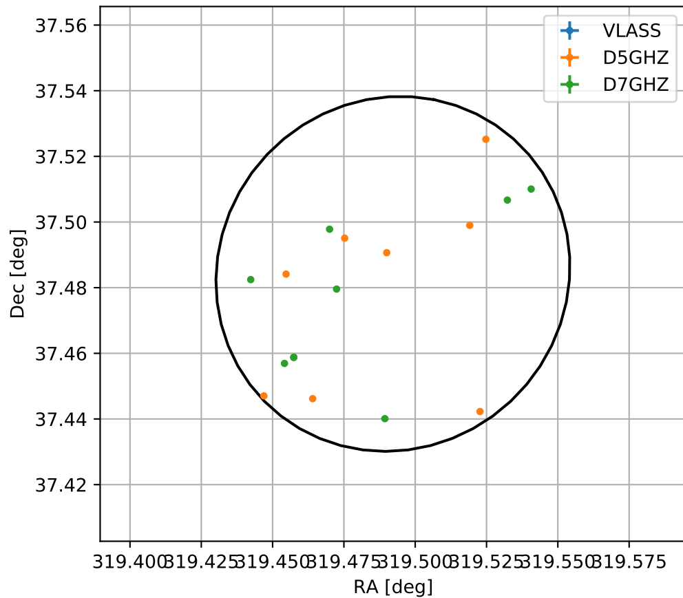
4FGL J2117.9+3729
