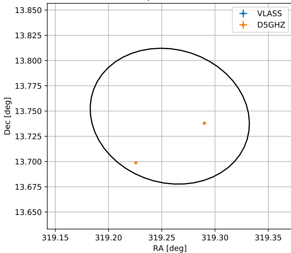
4FGL J2117.0+1344
