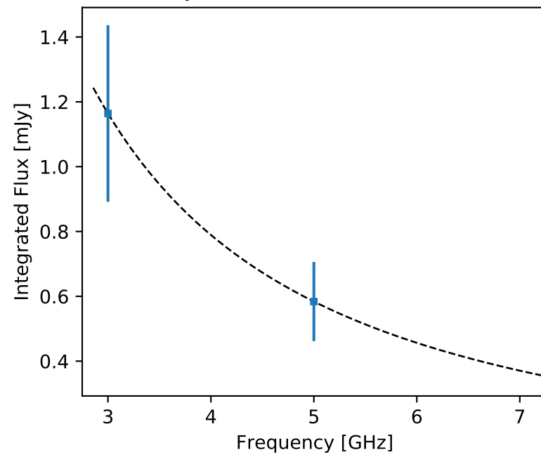
F357 J211709.59+134416.1 (unr)
