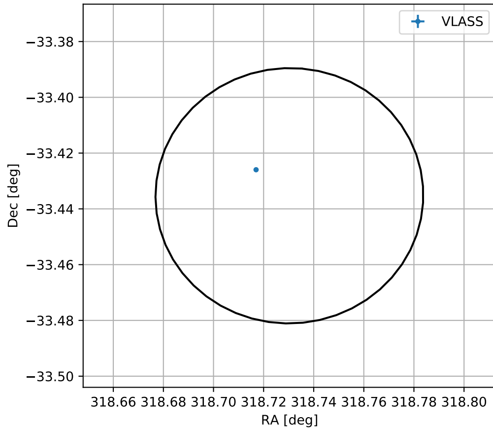
4FGL J2114.9-3326
