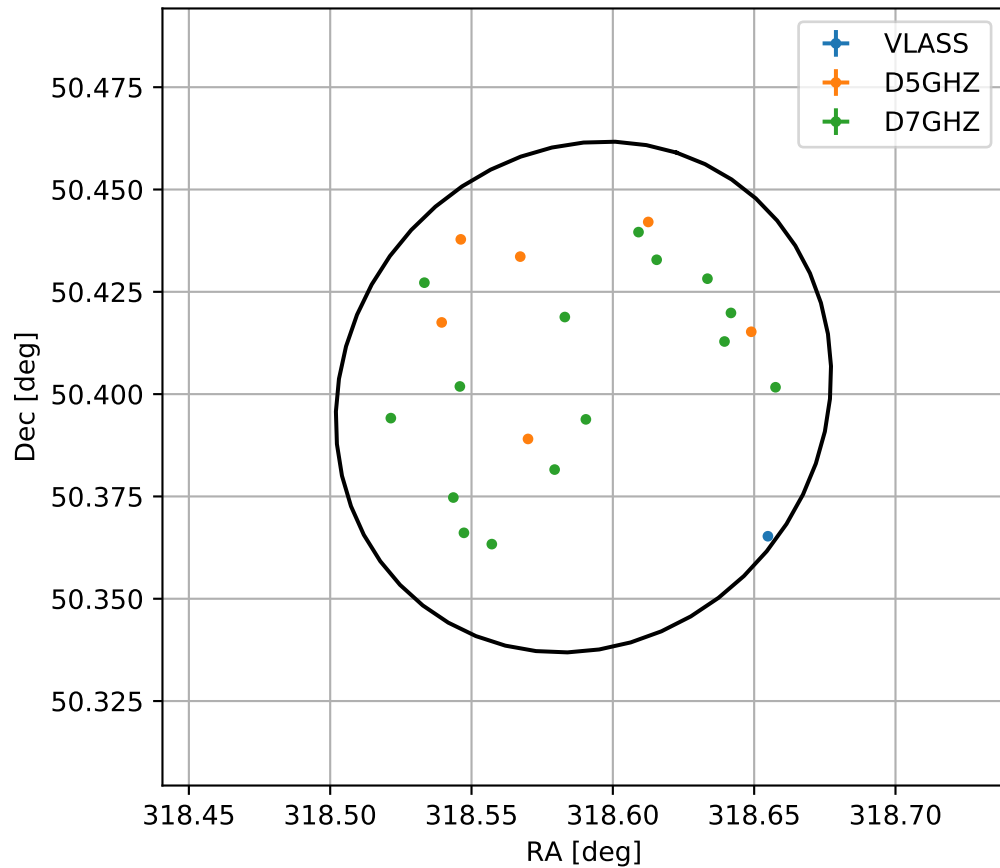
4FGL J2114.3+5023
