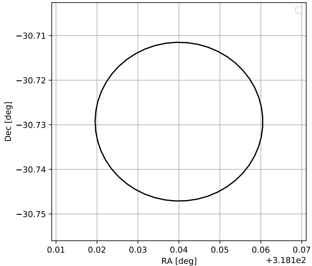
4FGL J2112.5-3043
