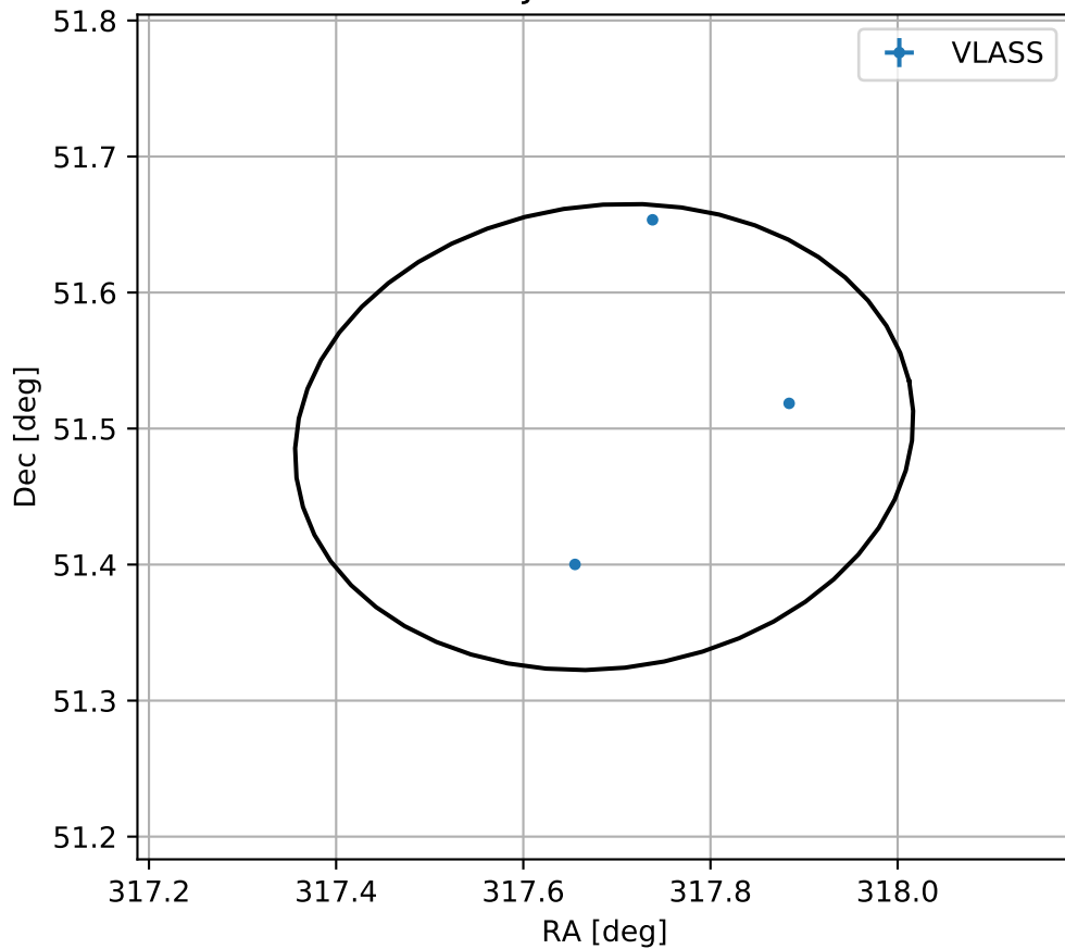
4FGL J2110.7+5129
