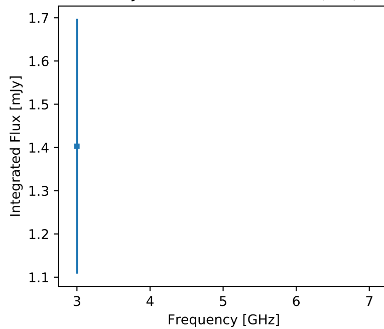
F357 J211132.17+513106.6 (unr)
