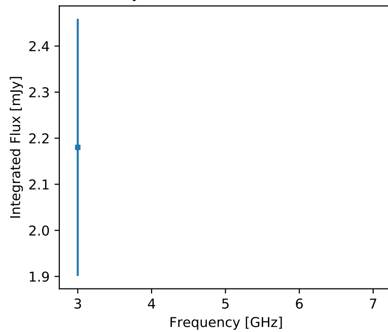
F357 J211057.14+513912.4 (unr)
