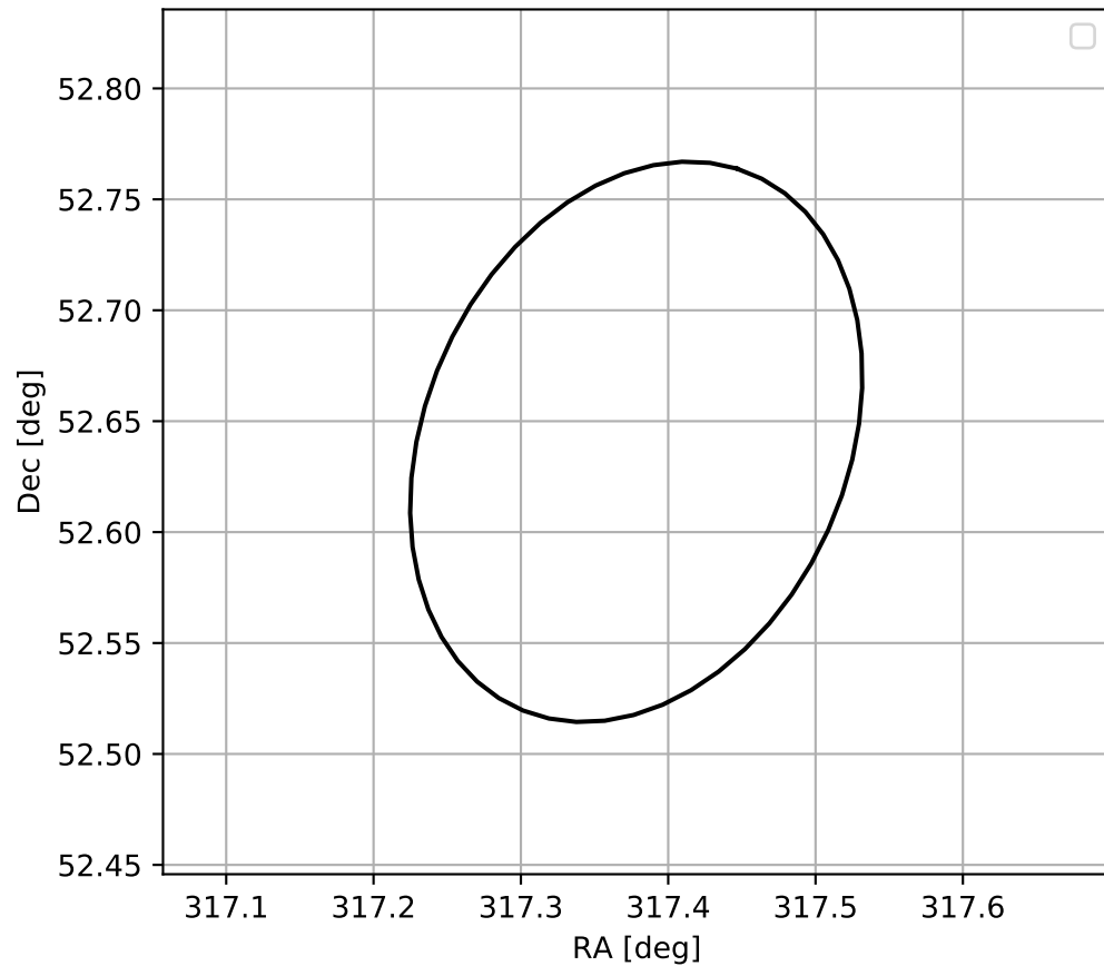
4FGL J2109.5+5238c
