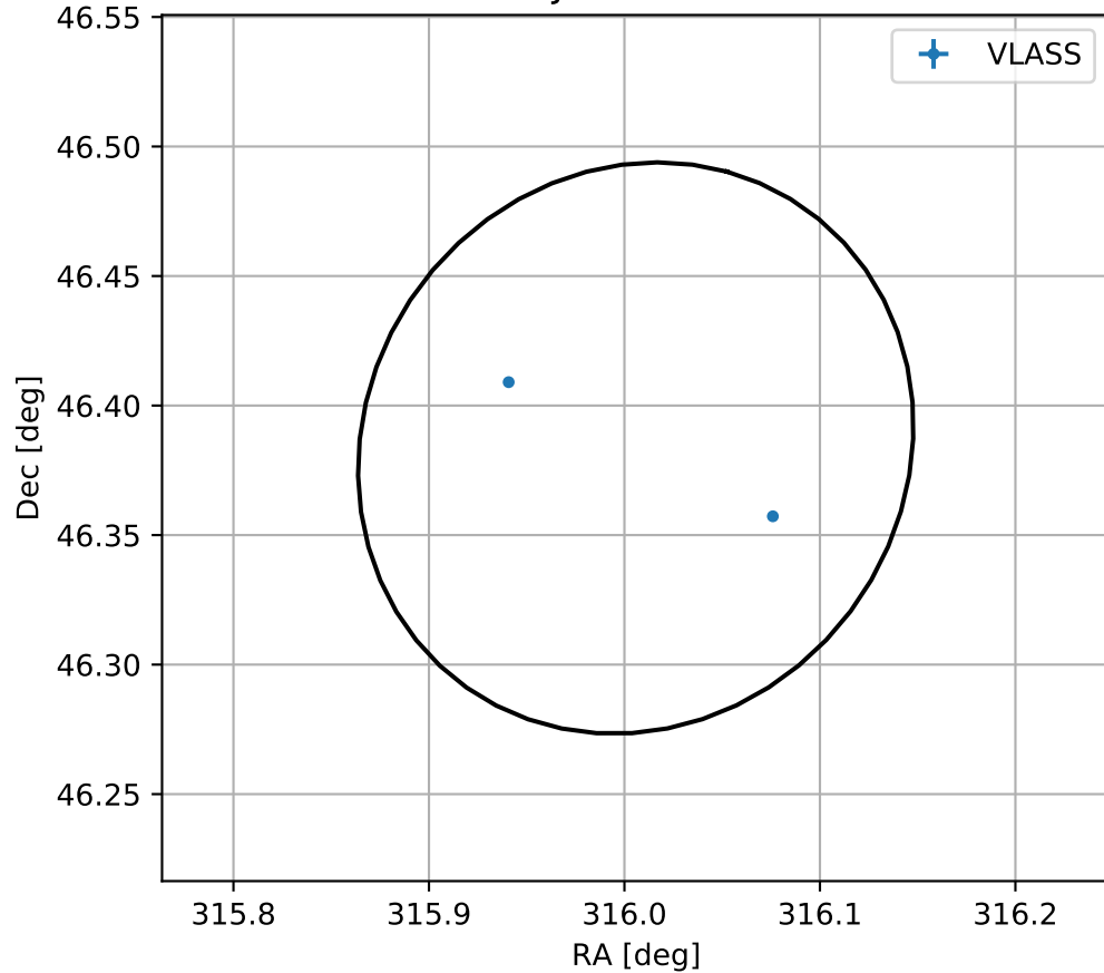
4FGL J2104.0+4623
