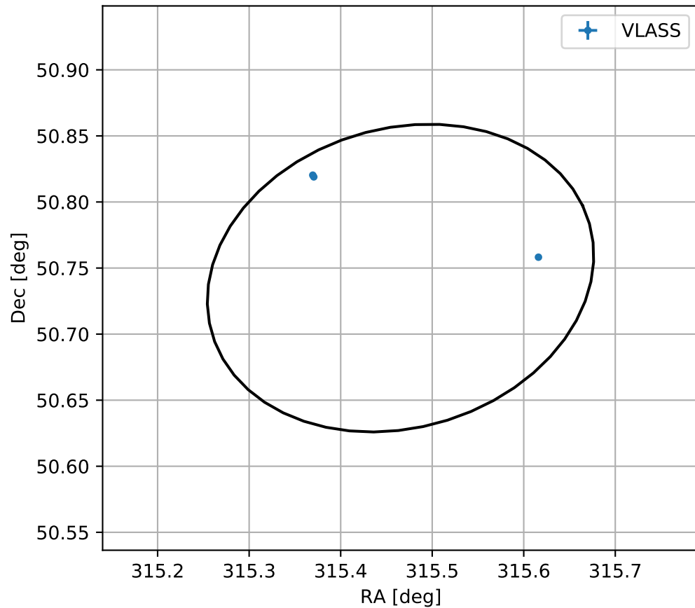
4FGL J2101.8+5044c
