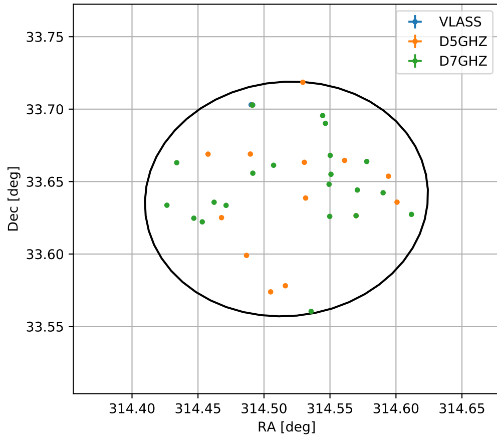
4FGL J2058.0+3338
