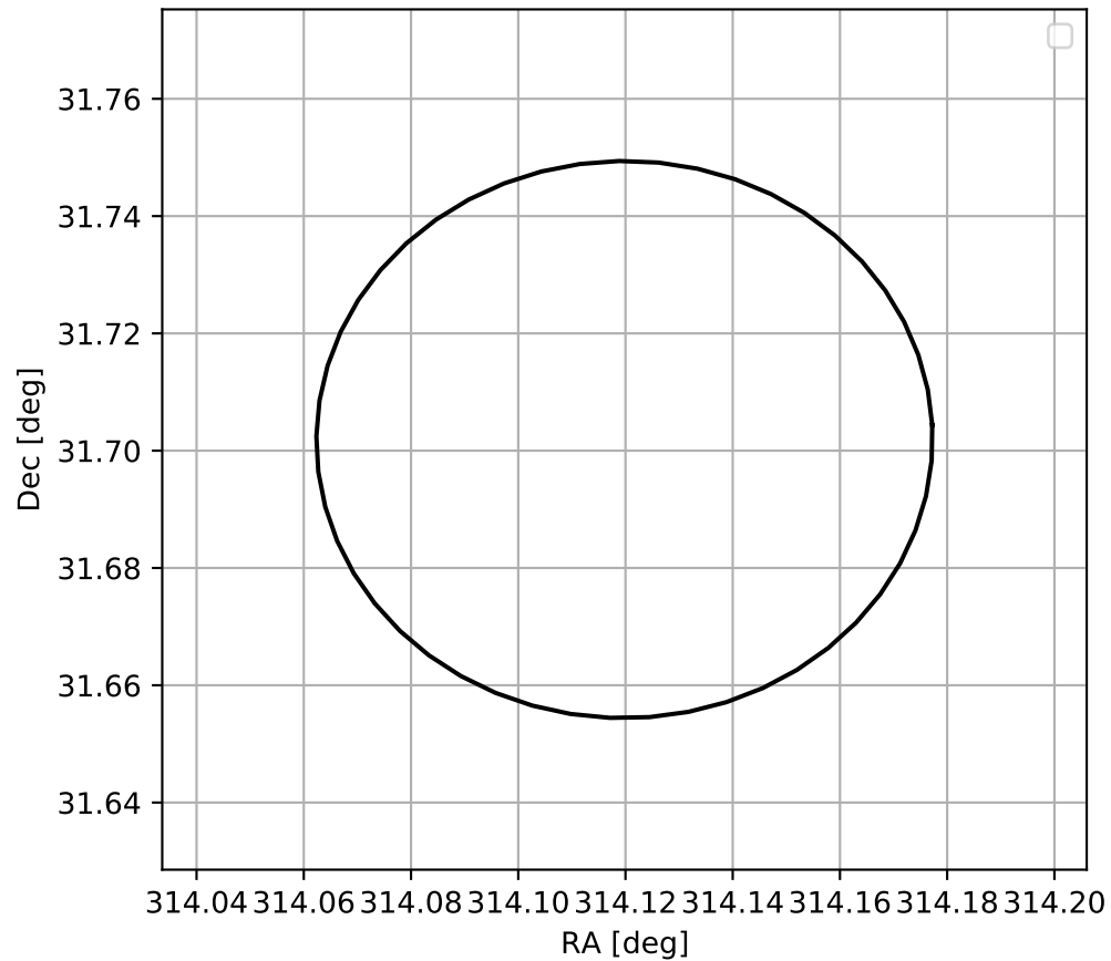
4FGL J2056.4+3142
