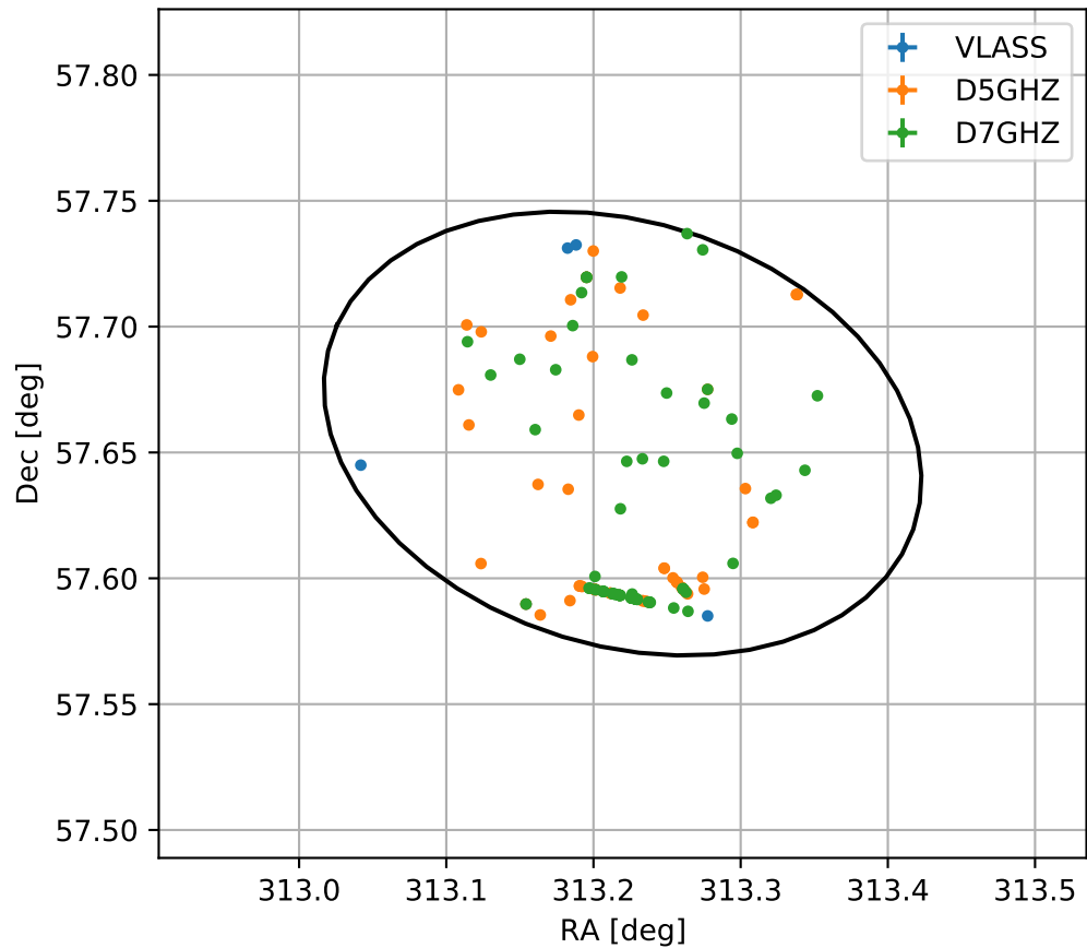
4FGL J2052.8+5739
