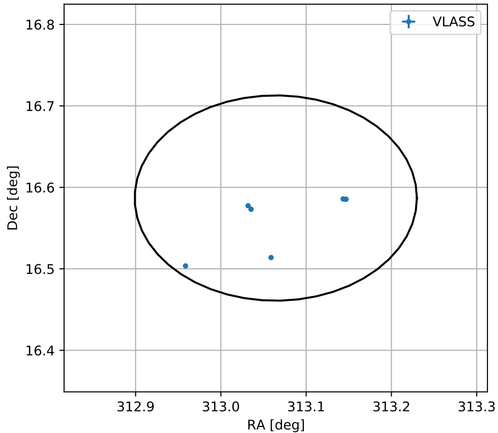
4FGL J2052.2+1635
