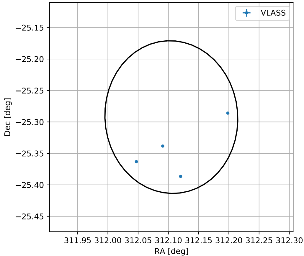
4FGL J2048.4-2517
