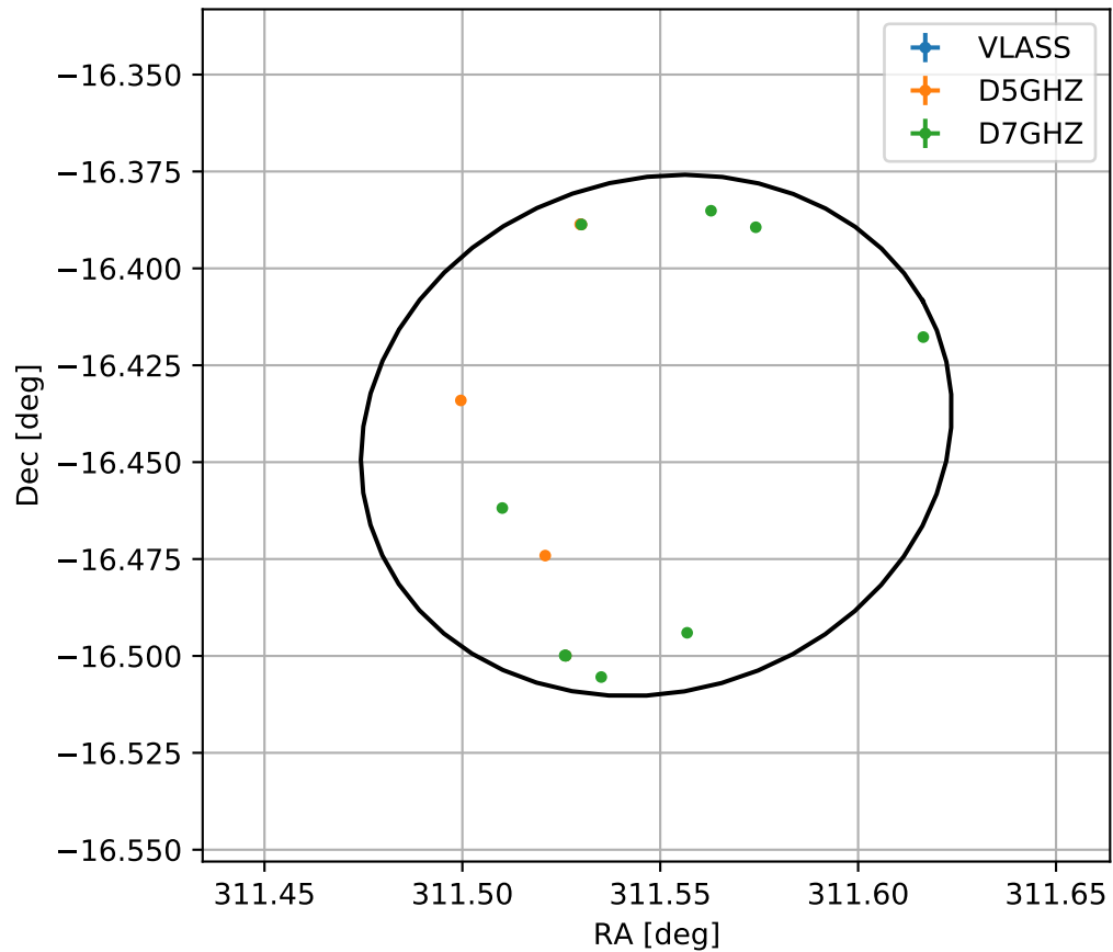
4FGL J2046.1-1626
