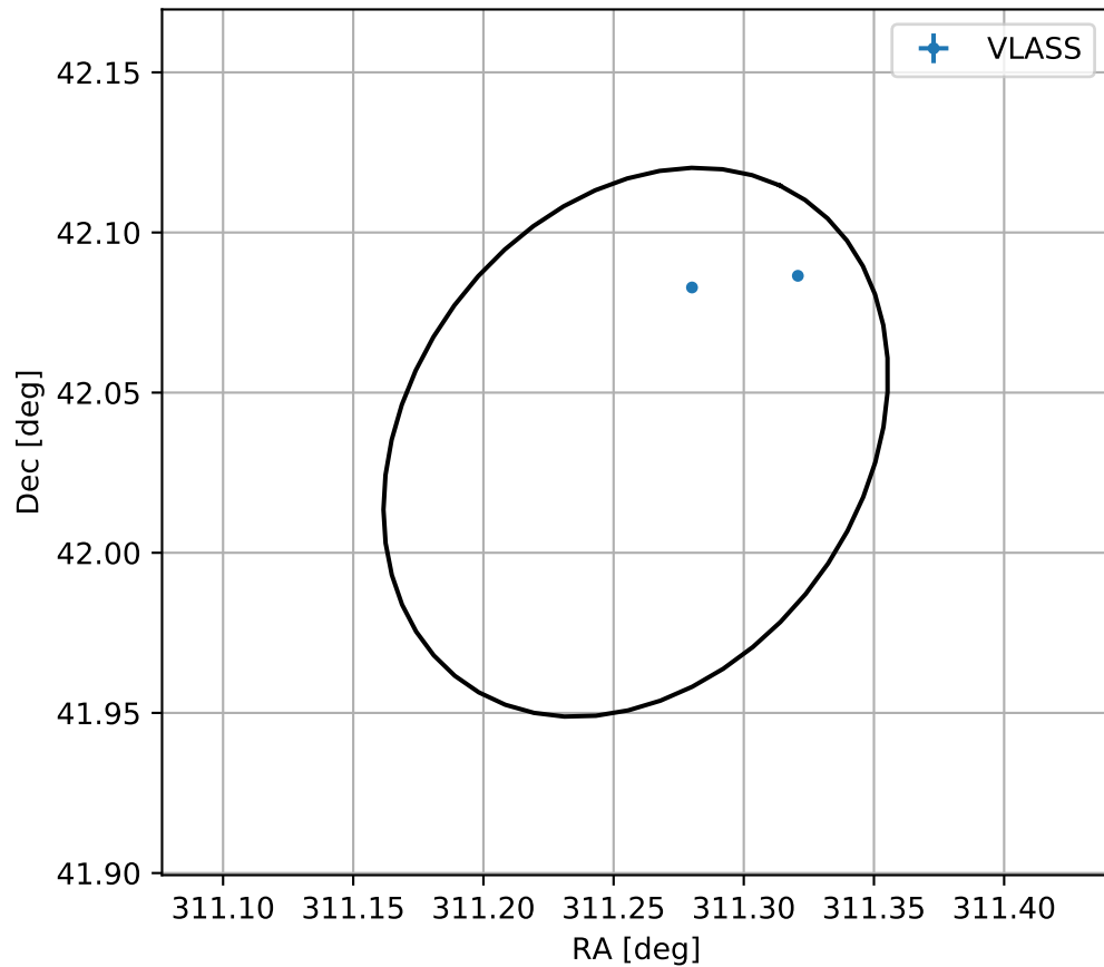
4FGL J2045.0+4202
