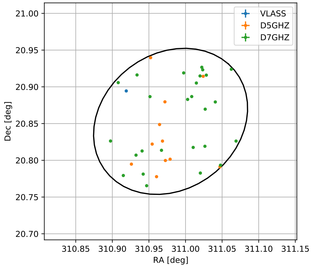
4FGL J2043.9+2051
