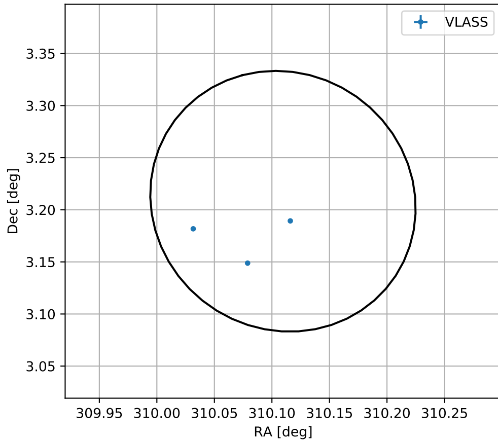
4FGL J2040.4+0312
