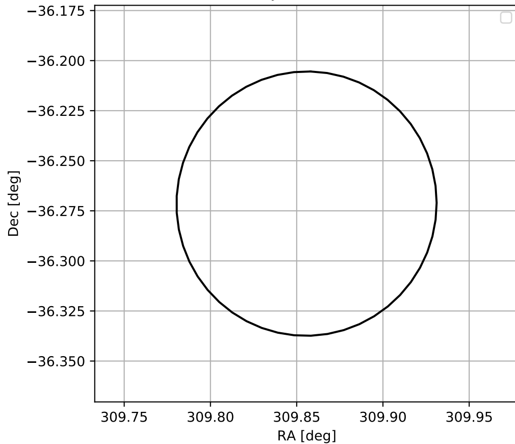
4FGL J2039.4-3616
